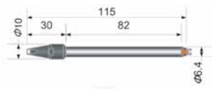
TB/SB Cartridge
