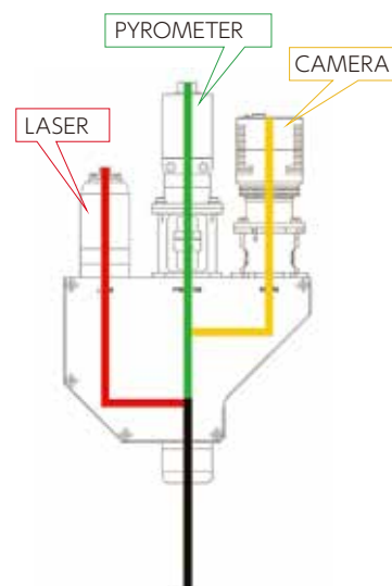
【 Inner drawing of the coaxial head 】
