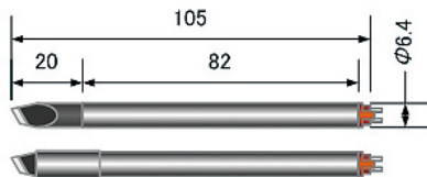
TS/DS/DN Cartridge
