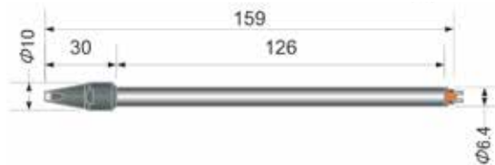
MB/DB Cartridge
