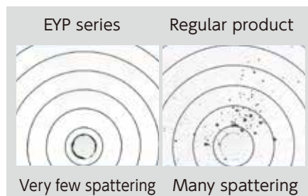
■ Solder wire
